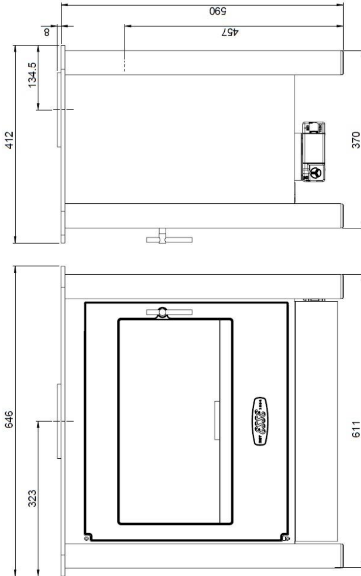
Fig 1a – G225L Dimensions
