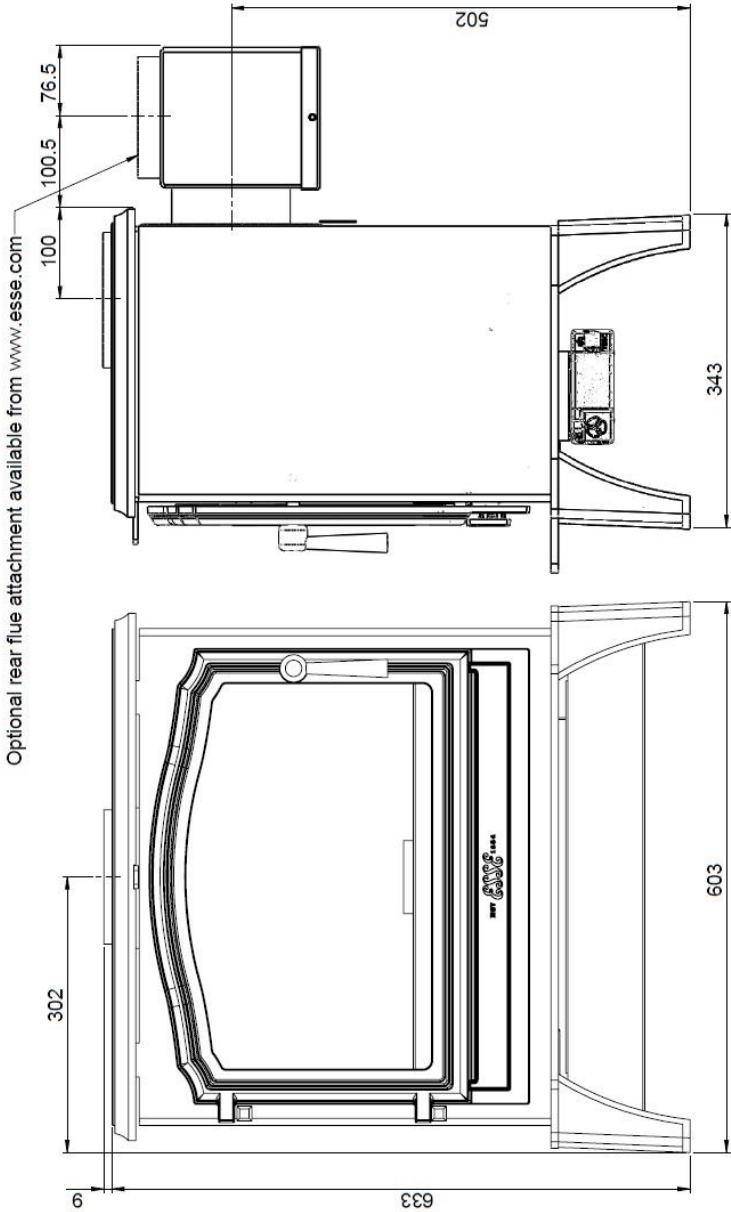
Fig 1b – G200L Dimensions
